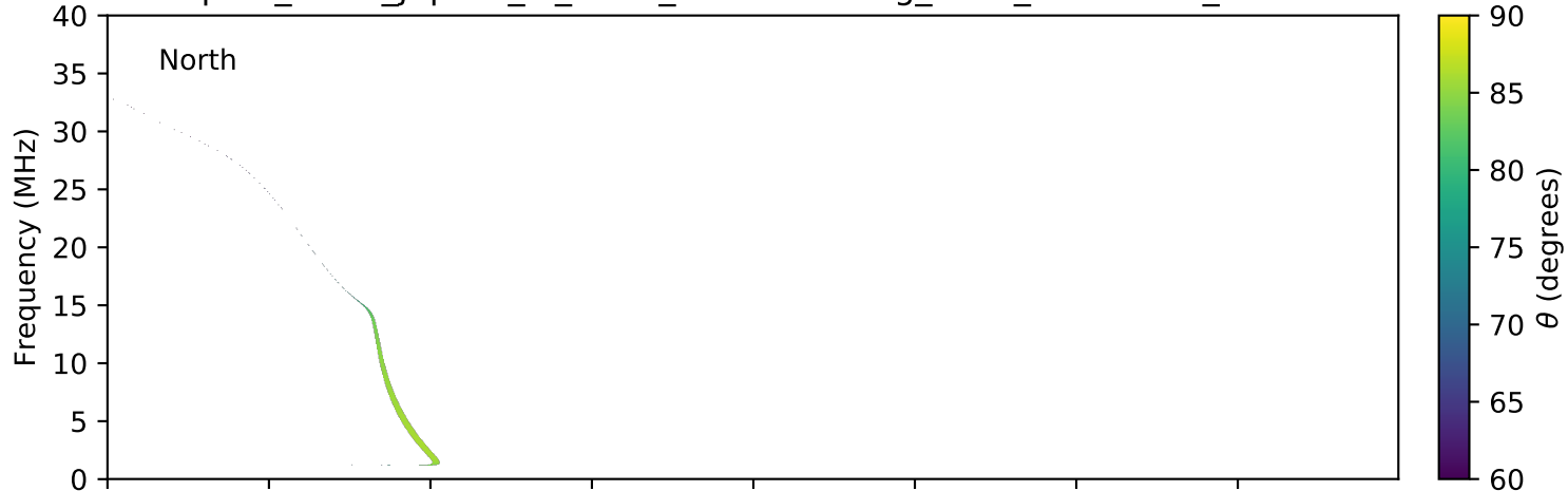
expres_earth_jupiter_io_isaac_lossc-wid1deg_1kev_20161204_v01.cdf
