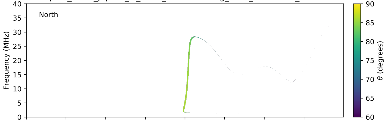
expres_earth_jupiter_io_isaac_lossc-wid1deg_1kev_20161203_v01.cdf
