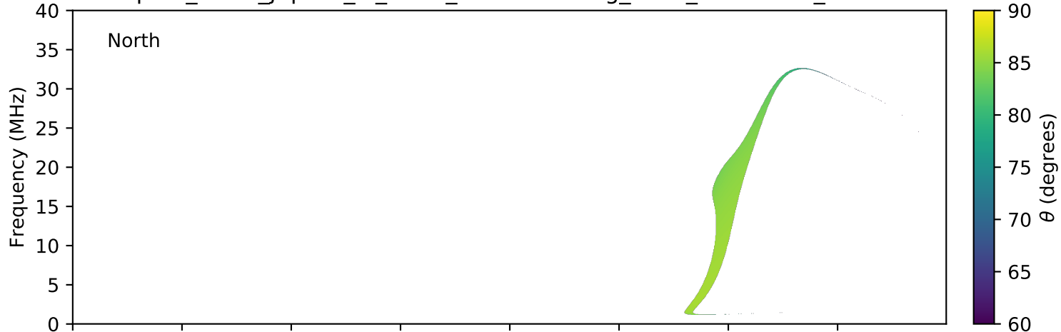
expres_earth_jupiter_io_isaac_lossc-wid1deg_1kev_20161201_v01.cdf
