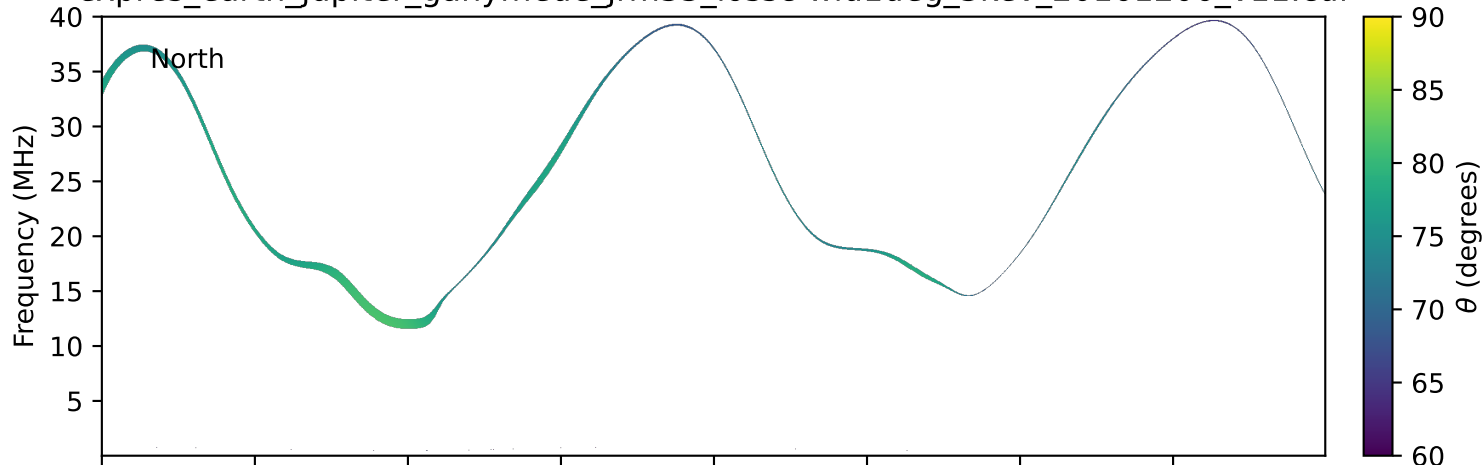
expres_earth_jupiter_ganymede_jrm33_lossc-wid1deg_3kev_20161206_v11.cdf
