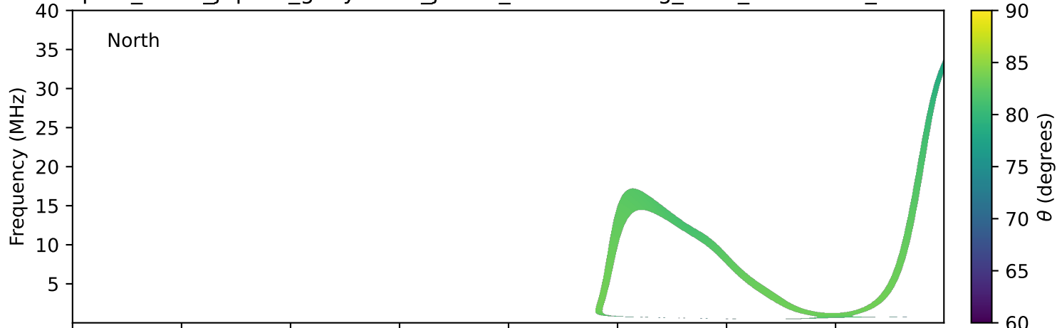
expres_earth_jupiter_ganymede_jrm33_lossc-wid1deg_3kev_20161205_v11.cdf
