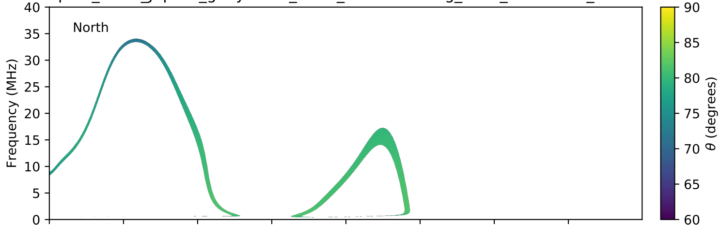
expres_earth_jupiter_ganymede_isaac_lossc-wid1deg_5kev_20161201_v01.cdf
