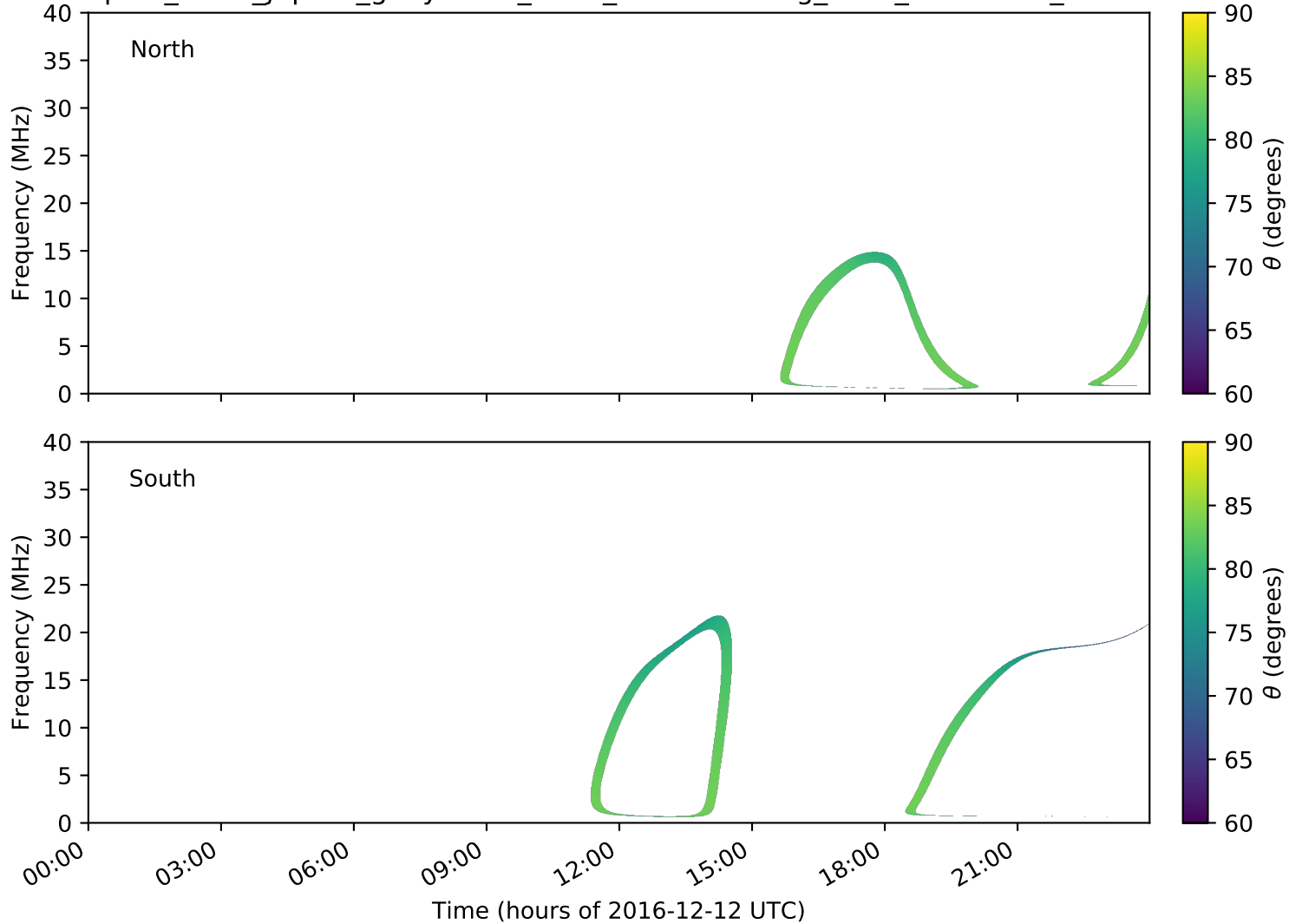
expres_earth_jupiter_ganymede_isaac_lossc-wid1deg_3kev_20161212_v01.cdf
