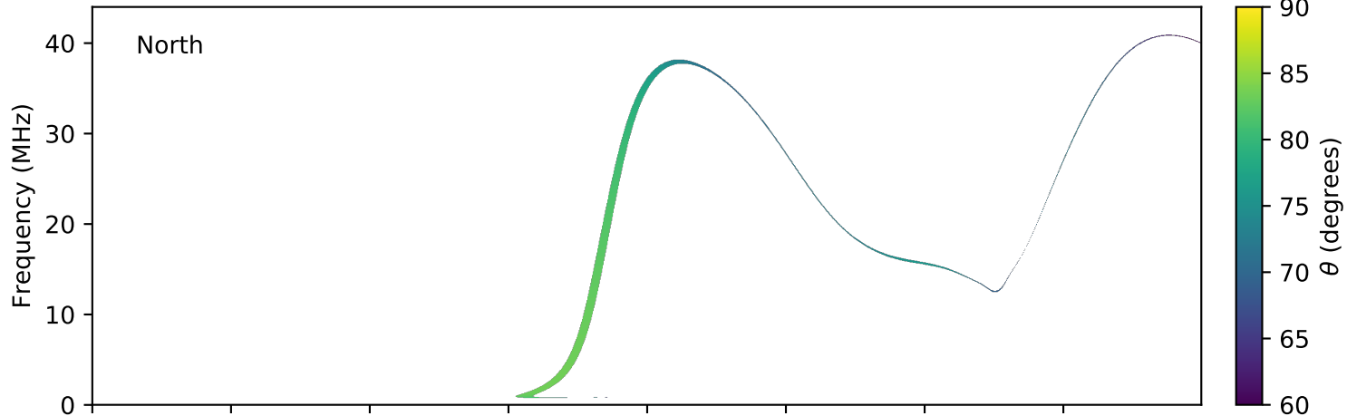
expres_earth_jupiter_europa_jrm09_lossc-wid1deg_3kev_20161227_v01.cdf
