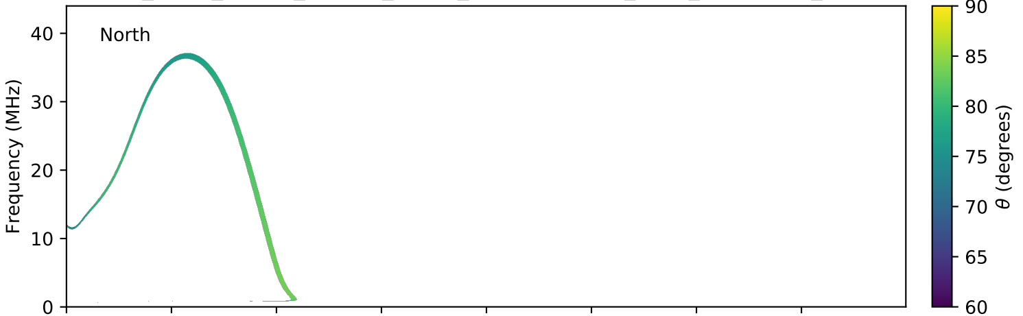
expres_earth_jupiter_europa_jrm09_lossc-wid1deg_3kev_20161225_v01.cdf
