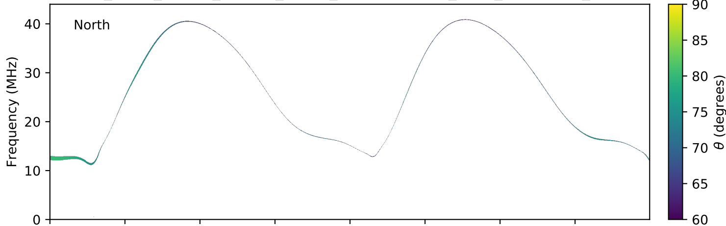
expres_earth_jupiter_europa_jrm09_lossc-wid1deg_3kev_20161224_v01.cdf
