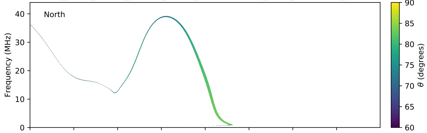
expres_earth_jupiter_europa_jrm09_lossc-wid1deg_3kev_20161214_v01.cdf
