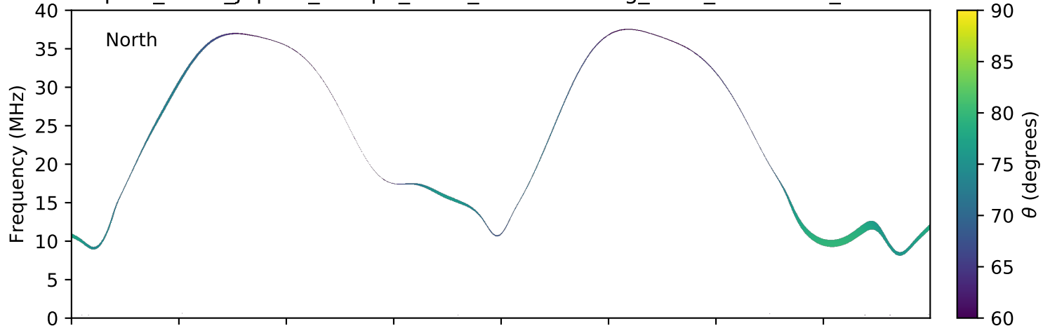
expres_earth_jupiter_europa_isaac_lossc-wid1deg_5kev_20161217_v01.cdf
