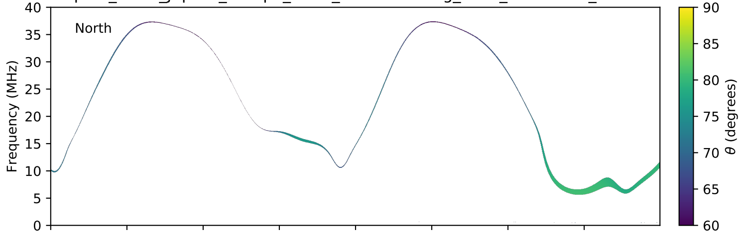
expres_earth_jupiter_europa_isaac_lossc-wid1deg_5kev_20161210_v01.cdf
