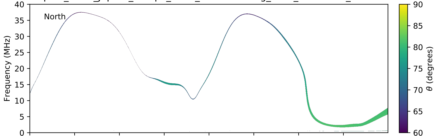
expres_earth_jupiter_europa_isaac_lossc-wid1deg_5kev_20161203_v01.cdf
