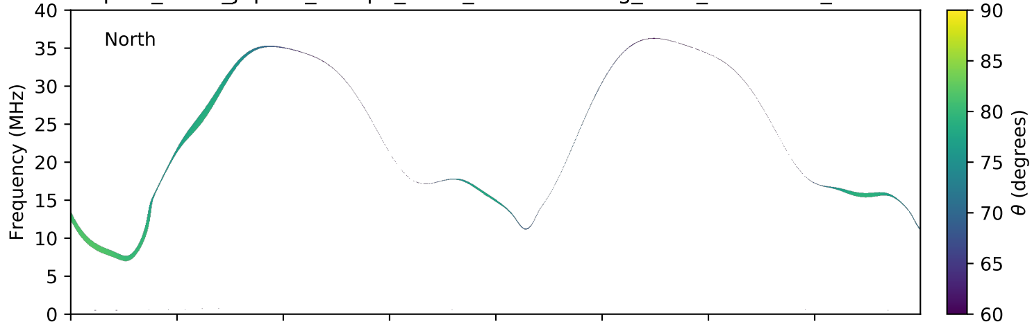
expres_earth_jupiter_europa_isaac_lossc-wid1deg_3kev_20161231_v01.cdf
