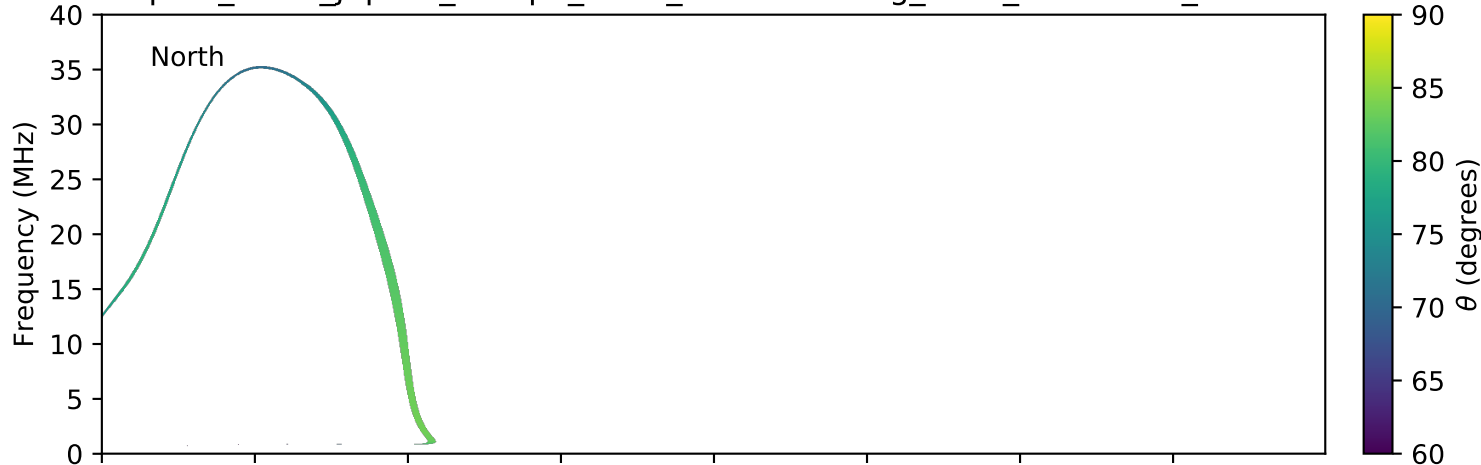
expres_earth_jupiter_europa_isaac_lossc-wid1deg_3kev_20161225_v01.cdf
