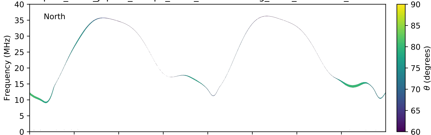
expres_earth_jupiter_europa_isaac_lossc-wid1deg_3kev_20161224_v01.cdf
