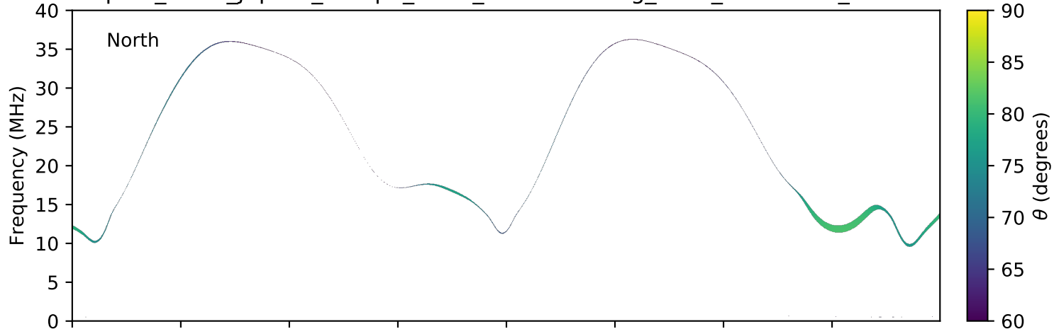
expres_earth_jupiter_europa_isaac_lossc-wid1deg_3kev_20161217_v01.cdf
