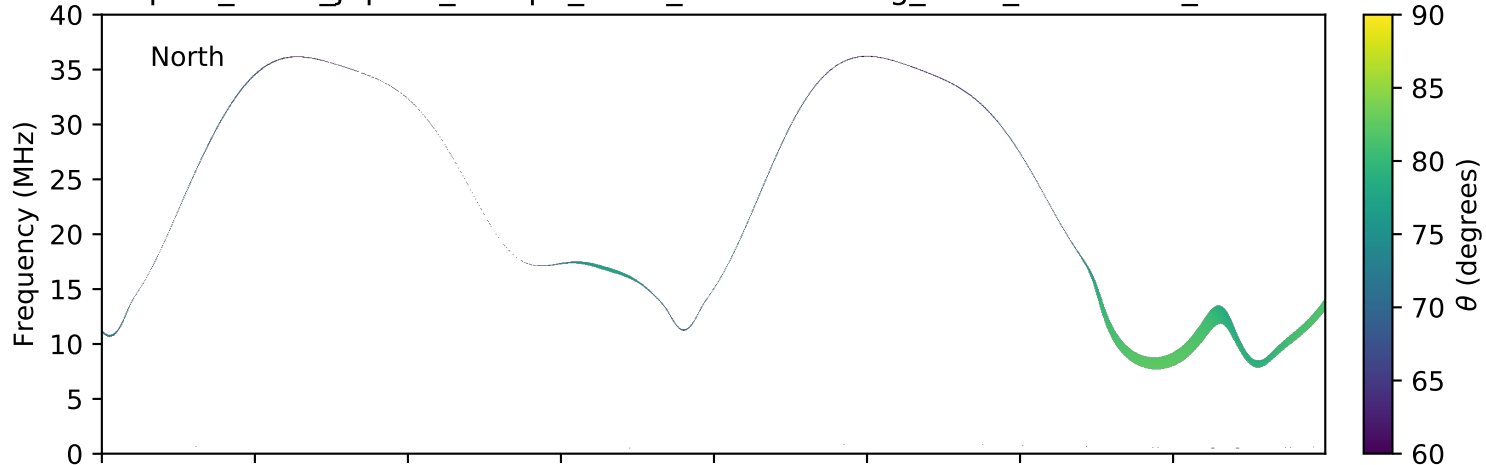
expres_earth_jupiter_europa_isaac_lossc-wid1deg_3kev_20161210_v01.cdf
