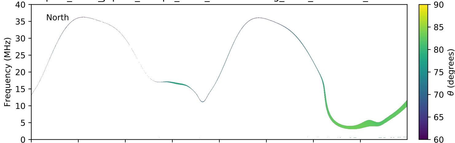
expres_earth_jupiter_europa_isaac_lossc-wid1deg_3kev_20161203_v01.cdf
