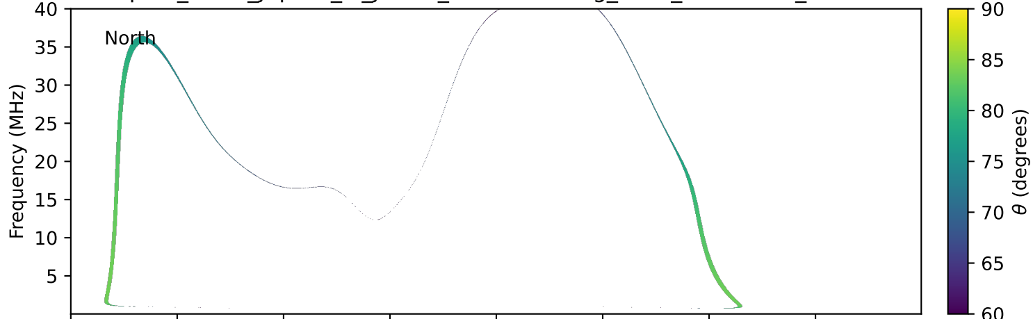
expres_earth_jupiter_io_jrm33_lossc-wid1deg_3kev_20161119_v11.cdf
