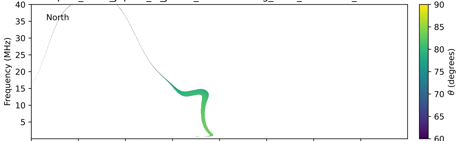
expres_earth_jupiter_io_jrm33_lossc-wid1deg_3kev_20161114_v11.cdf
