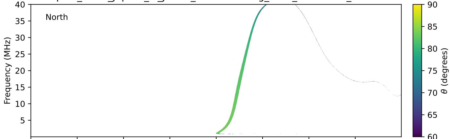
expres_earth_jupiter_io_jrm33_lossc-wid1deg_3kev_20161106_v11.cdf
