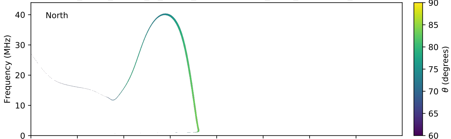
expres_earth_jupiter_io_jrm09_lossc-wid1deg_3kev_20161125_v01.cdf
