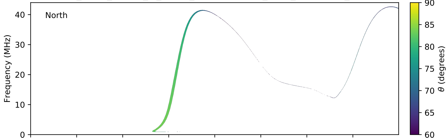
expres_earth_jupiter_io_jrm09_lossc-wid1deg_3kev_20161119_v01.cdf
