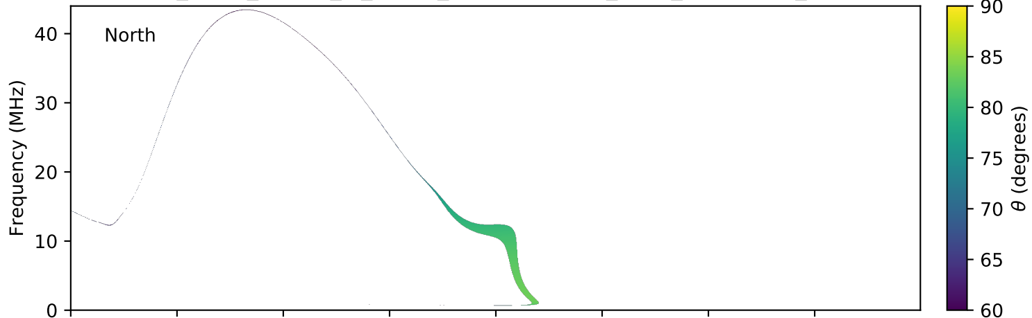
expres_earth_jupiter_io_jrm09_lossc-wid1deg_3kev_20161116_v01.cdf
