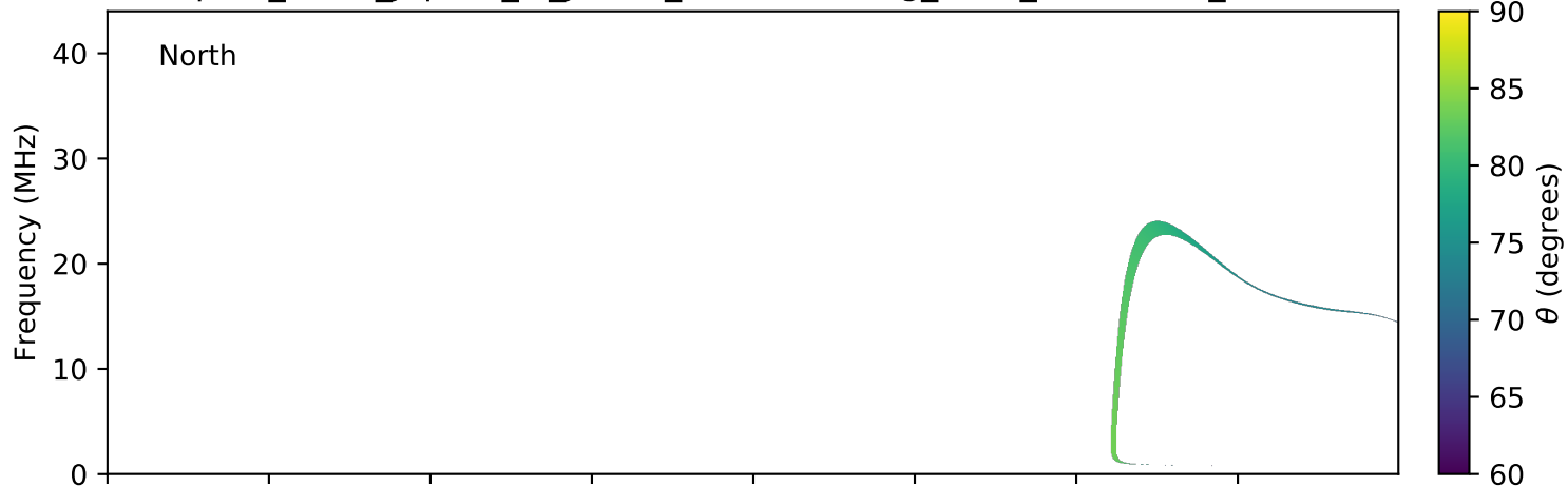
expres_earth_jupiter_io_jrm09_lossc-wid1deg_3kev_20161115_v01.cdf
