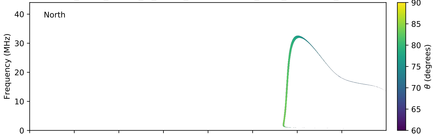
expres_earth_jupiter_io_jrm09_lossc-wid1deg_3kev_20161108_v01.cdf
