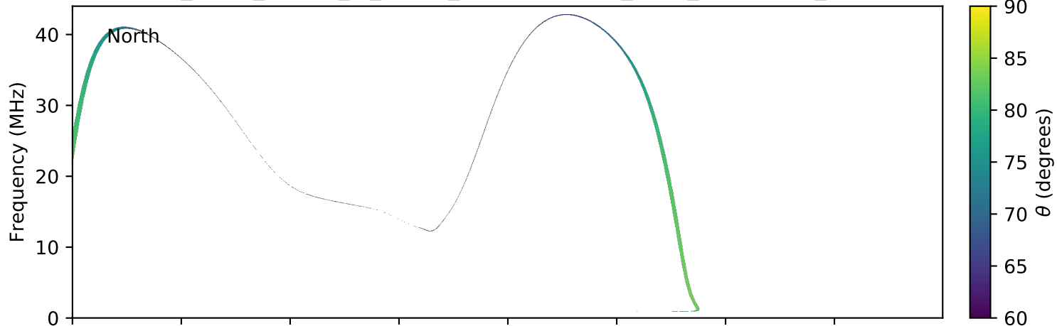
expres_earth_jupiter_io_jrm09_lossc-wid1deg_3kev_20161107_v01.cdf
