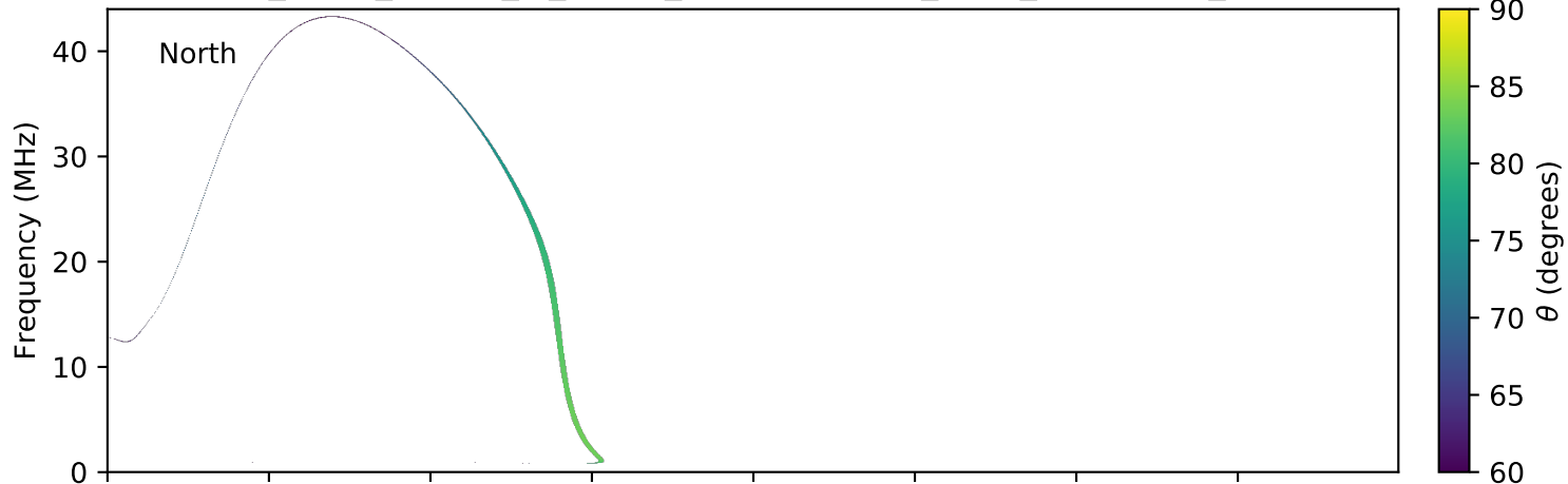
expres_earth_jupiter_io_jrm09_lossc-wid1deg_3kev_20161102_v01.cdf
