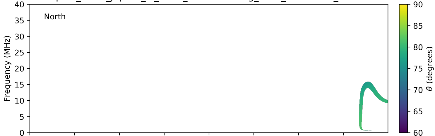
expres_earth_jupiter_io_isaac_lossc-wid1deg_5kev_20161129_v01.cdf
