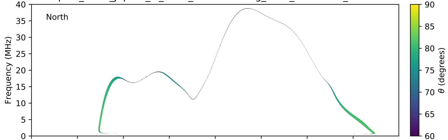
expres_earth_jupiter_io_isaac_lossc-wid1deg_5kev_20161128_v01.cdf
