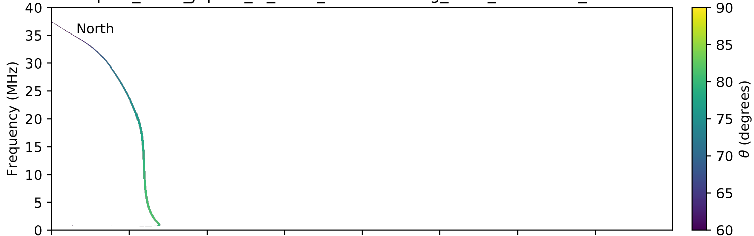
expres_earth_jupiter_io_isaac_lossc-wid1deg_5kev_20161127_v01.cdf
