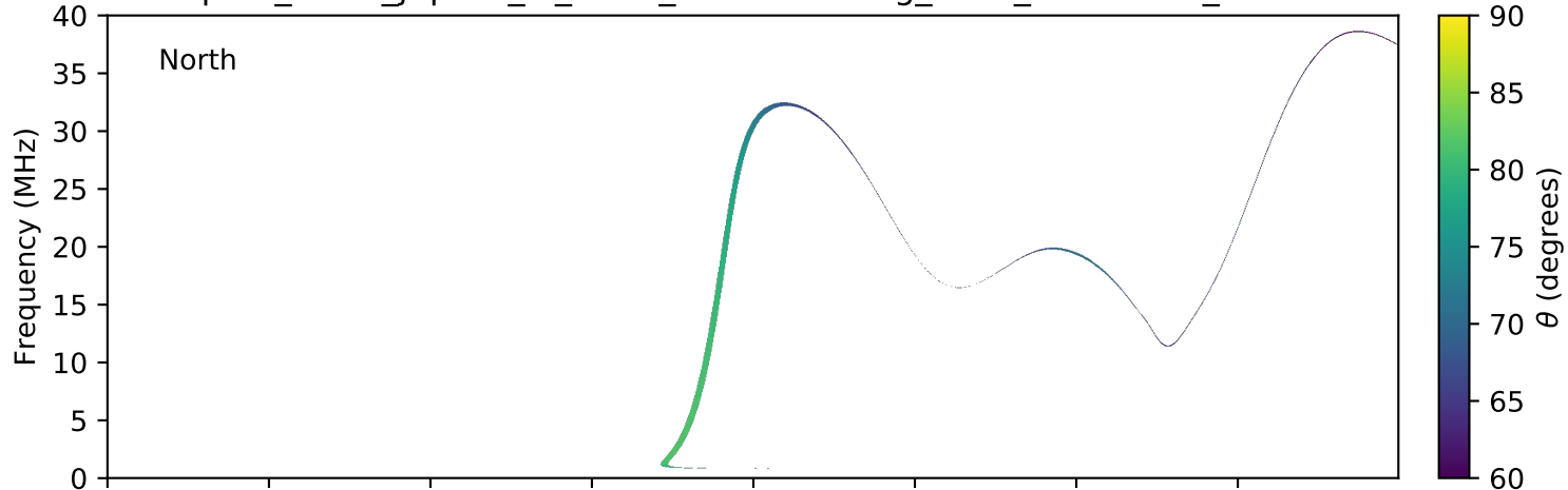
expres_earth_jupiter_io_isaac_lossc-wid1deg_5kev_20161126_v01.cdf
