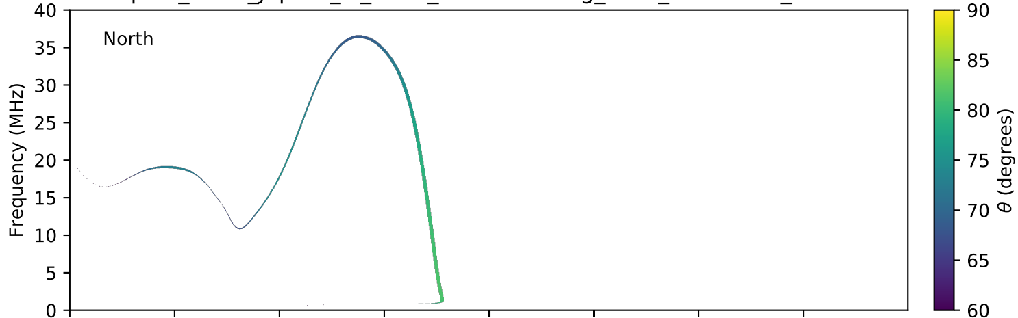
expres_earth_jupiter_io_isaac_lossc-wid1deg_5kev_20161125_v01.cdf
