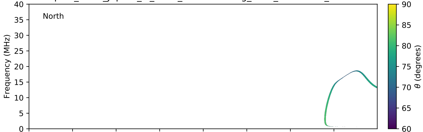
expres_earth_jupiter_io_isaac_lossc-wid1deg_5kev_20161122_v01.cdf
