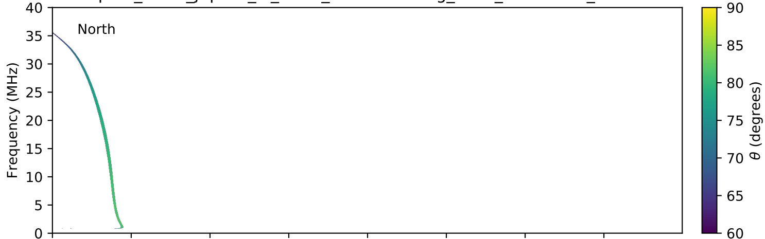
expres_earth_jupiter_io_isaac_lossc-wid1deg_5kev_20161120_v01.cdf
