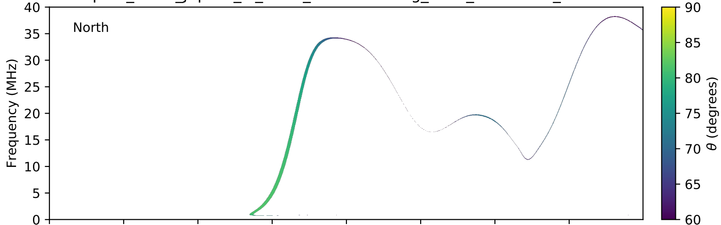
expres_earth_jupiter_io_isaac_lossc-wid1deg_5kev_20161119_v01.cdf
