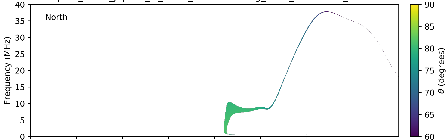
expres_earth_jupiter_io_isaac_lossc-wid1deg_5kev_20161117_v01.cdf
