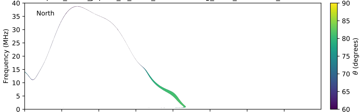
expres_earth_jupiter_io_isaac_lossc-wid1deg_5kev_20161116_v01.cdf
