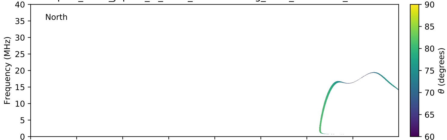
expres_earth_jupiter_io_isaac_lossc-wid1deg_5kev_20161115_v01.cdf
