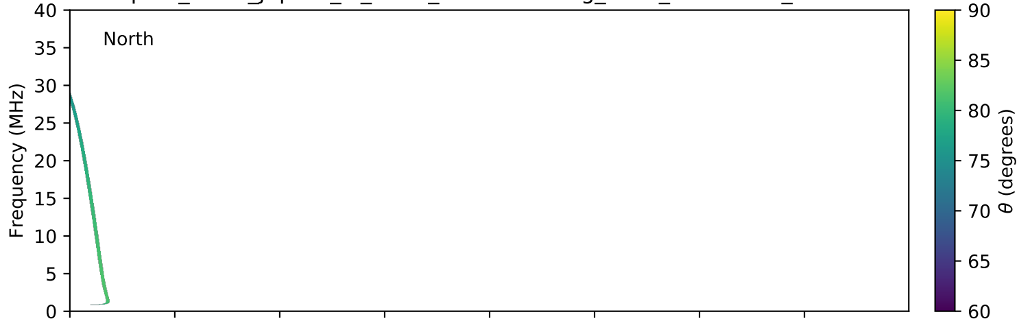
expres_earth_jupiter_io_isaac_lossc-wid1deg_5kev_20161113_v01.cdf
