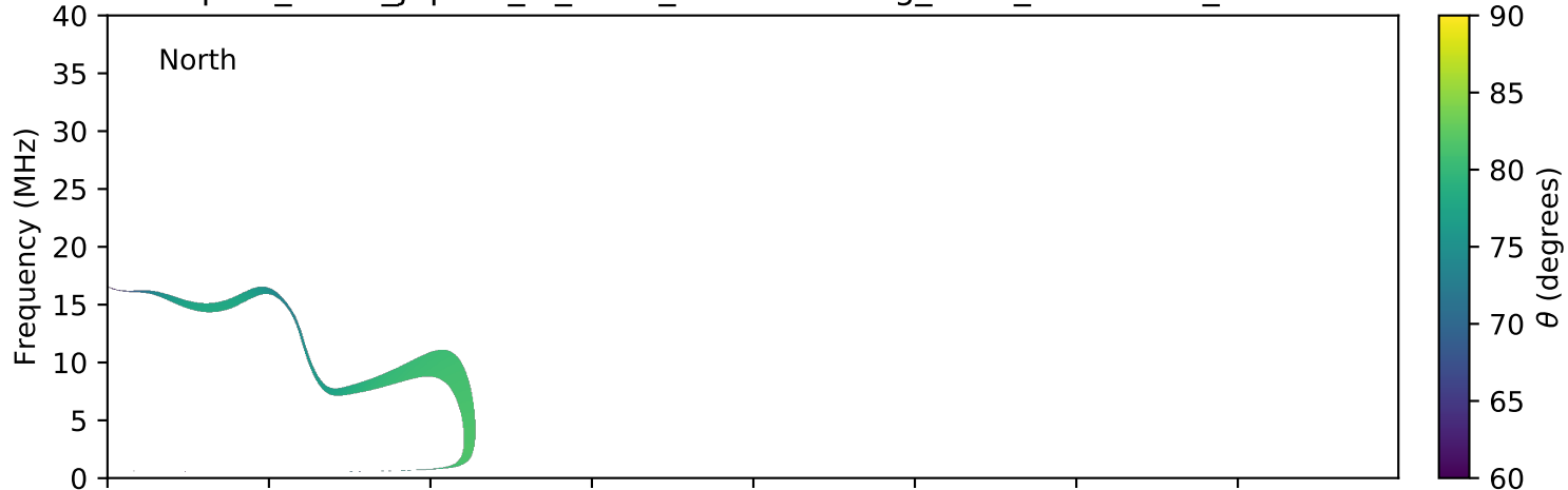
expres_earth_jupiter_io_isaac_lossc-wid1deg_5kev_20161111_v01.cdf
