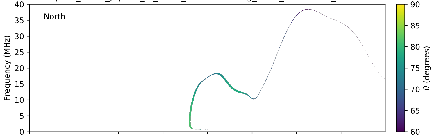
expres_earth_jupiter_io_isaac_lossc-wid1deg_5kev_20161110_v01.cdf
