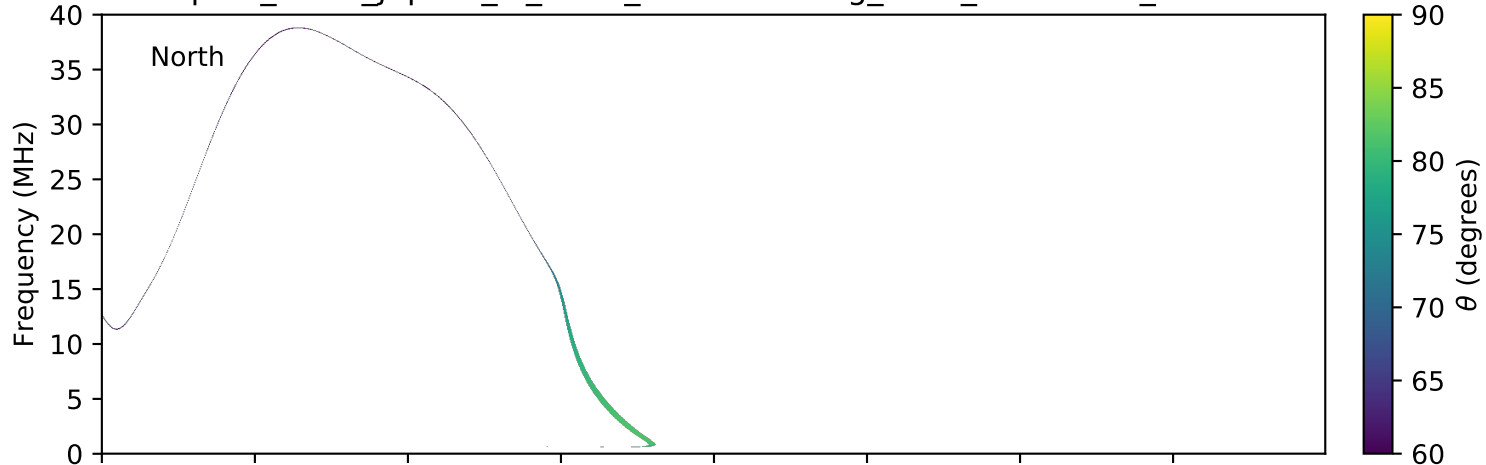
expres_earth_jupiter_io_isaac_lossc-wid1deg_5kev_20161109_v01.cdf
