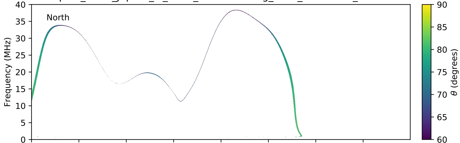
expres_earth_jupiter_io_isaac_lossc-wid1deg_5kev_20161107_v01.cdf
