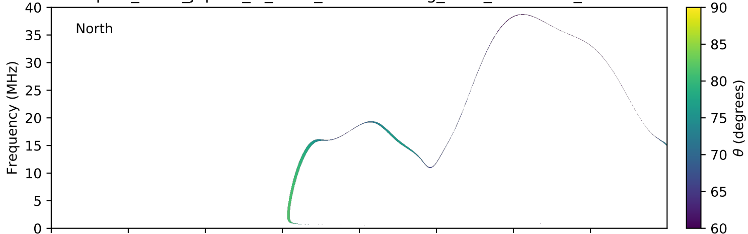
expres_earth_jupiter_io_isaac_lossc-wid1deg_5kev_20161103_v01.cdf
