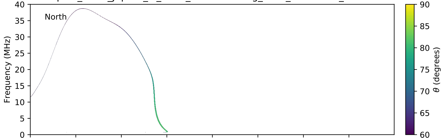
expres_earth_jupiter_io_isaac_lossc-wid1deg_5kev_20161102_v01.cdf
