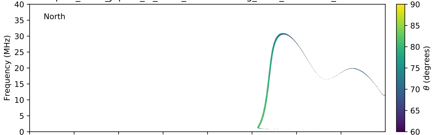
expres_earth_jupiter_io_isaac_lossc-wid1deg_5kev_20161101_v01.cdf
