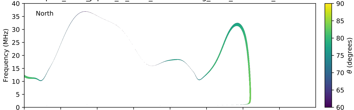
expres_earth_jupiter_io_isaac_lossc-wid1deg_3kev_20161130_v01.cdf
